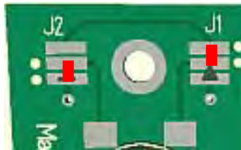
Solder pads J_1 and J_2 connection for heat flux direction (standard delivered)
