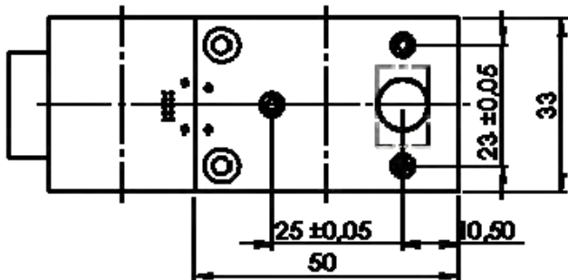
TE-CORE /RF (bottom view) position for drillings
