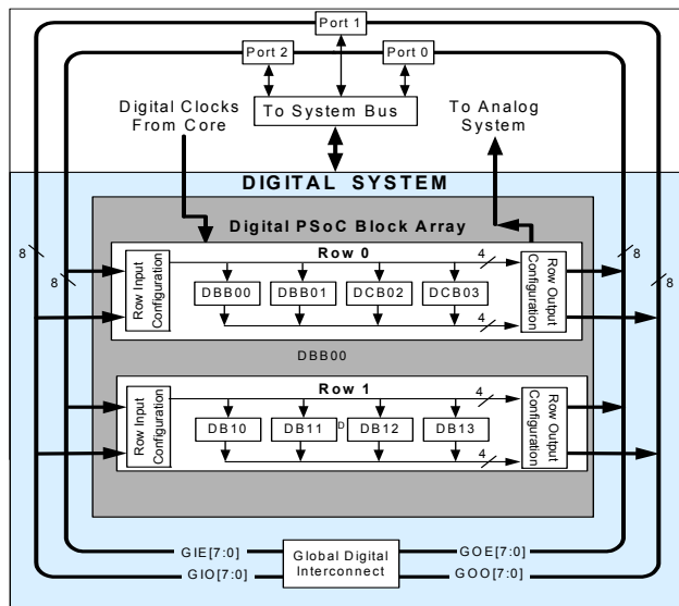
Figure 5-1. Digital System Block Diagram
