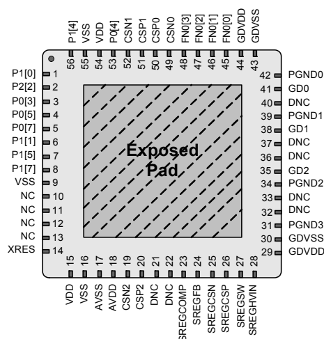
QFN Top View
