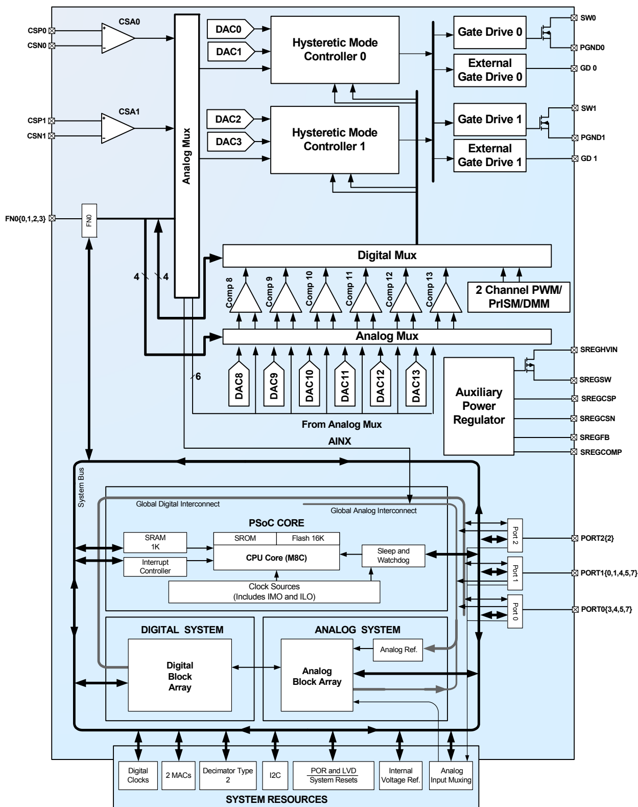
Figure 2-5. CY8CLED02D01 Logic Block Diagram
