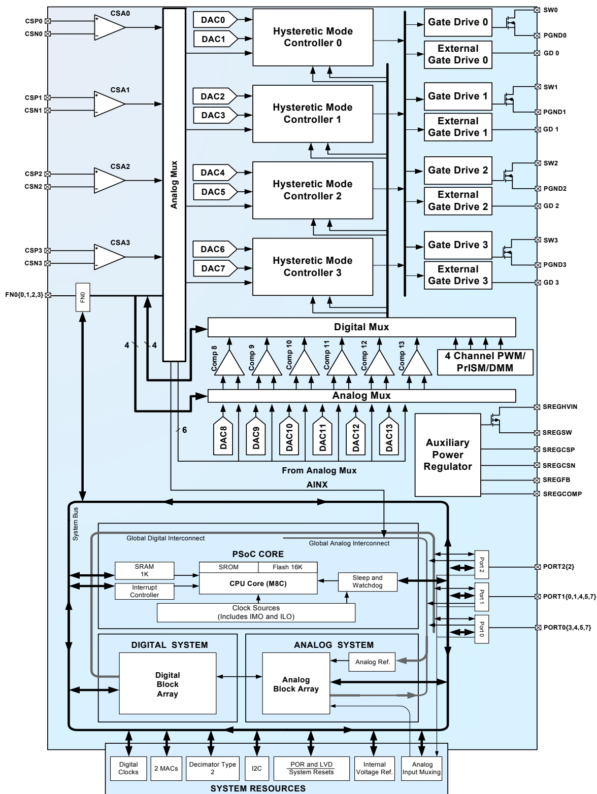
Figure 2-1. CY8CLED04D0x Logic Block Diagram
