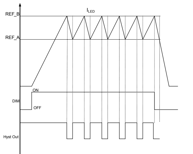
Figure 4-2. Current Waveforms
