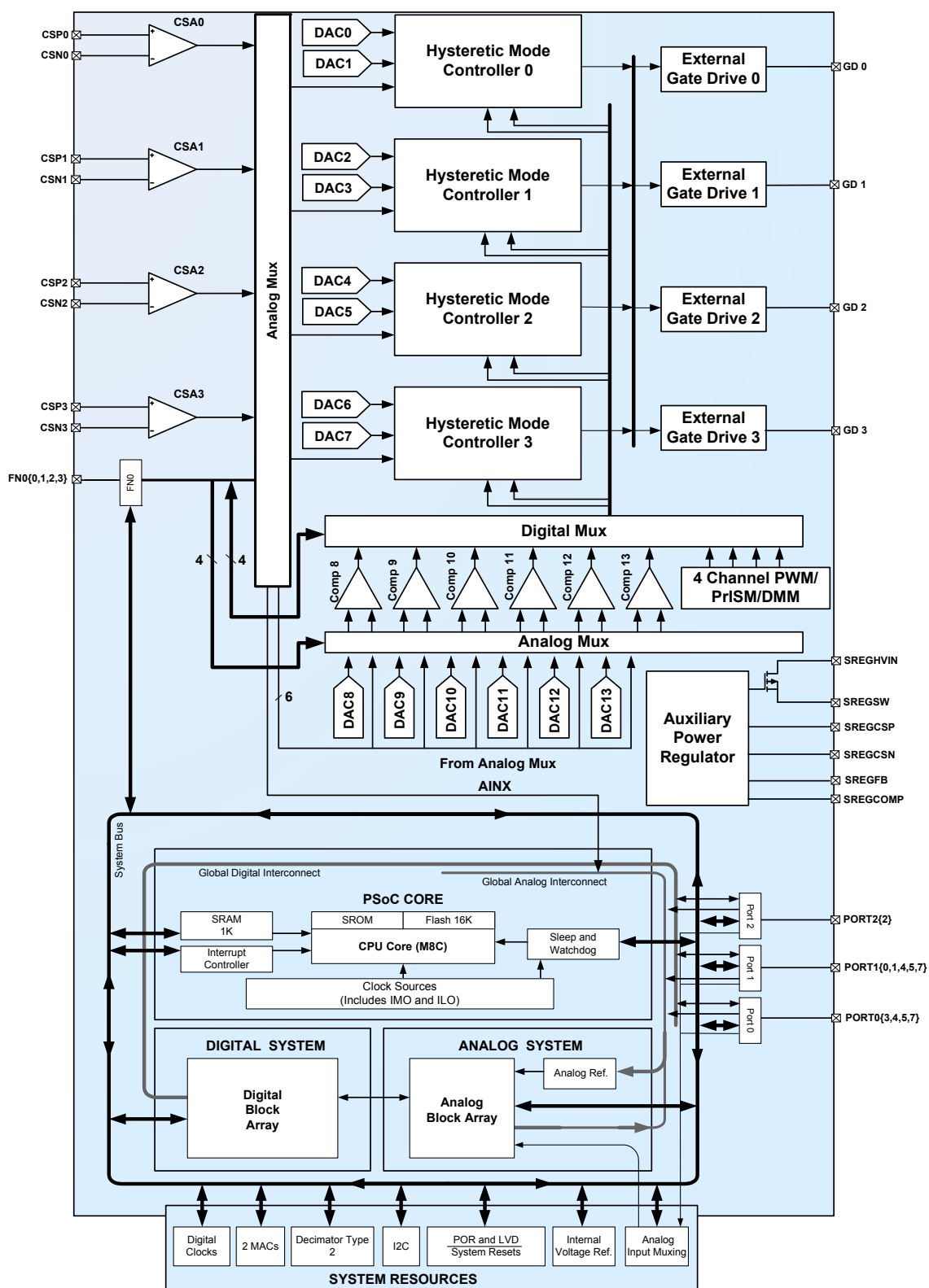
Figure 2-2. CY8CLED04G01 Logic Block Diagram
