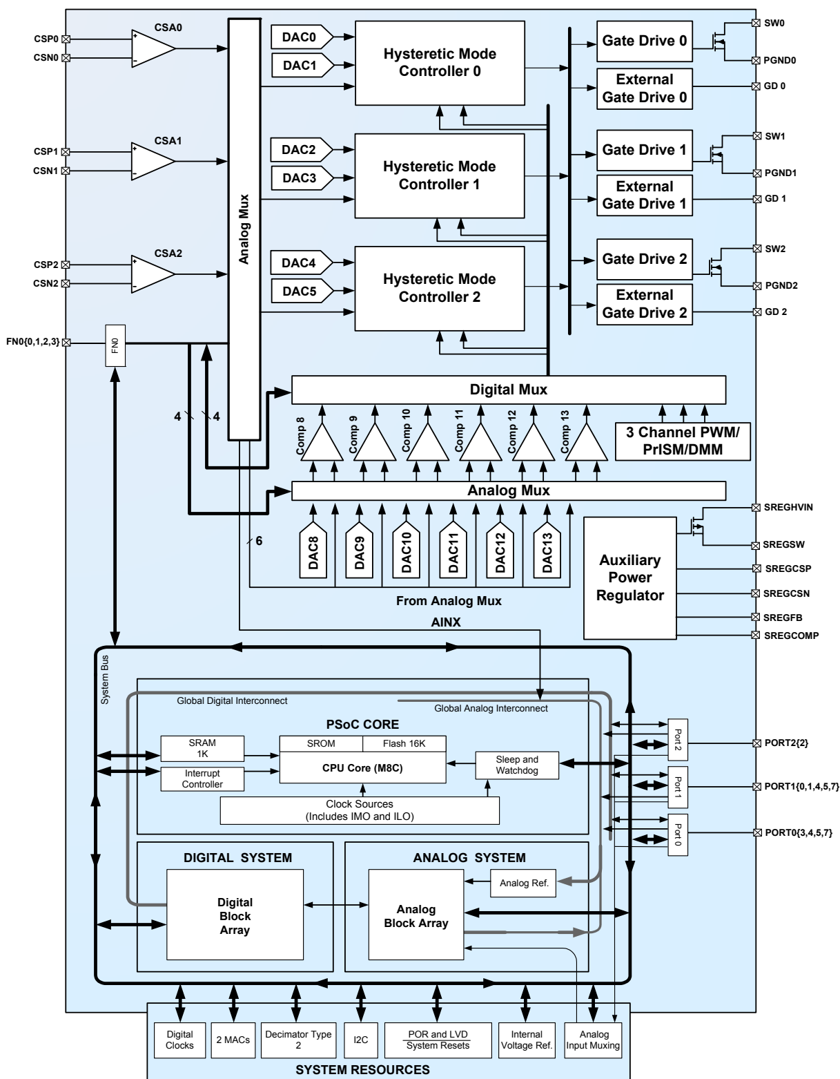
Figure 2-3. CY8CLED03D0x Logic Block Diagram
