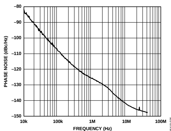
Figure 30. Internal VCO Phase Noise (Absolute) Direct to LVPECL at 2550 MHz
