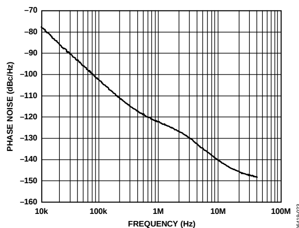
Figure 28. Internal VCO Phase Noise (Absolute) Direct to LVPECL at 2950 MHz
