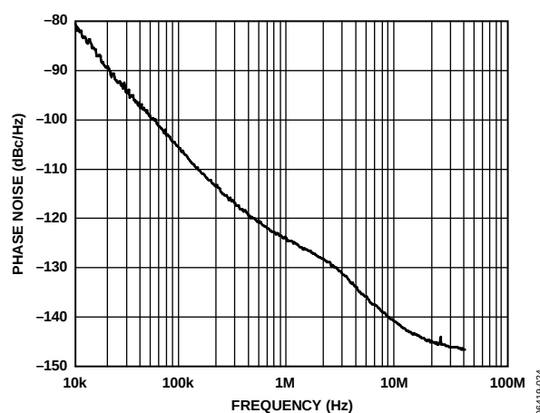
Figure 29. Internal VCO Phase Noise (Absolute) Direct to LVPECL at 2750 MHz
