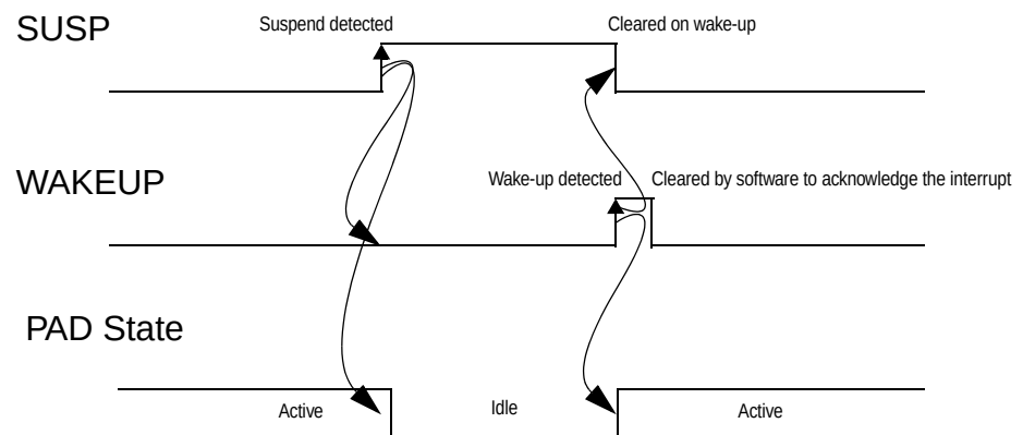
Figure 27-9. Pad Events
