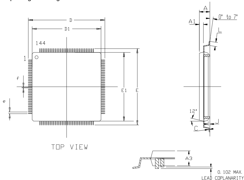
Figure 37-2. LQFP-144 package drawing
