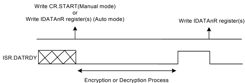
Figure 33-2. Manual and Automatic Modes when MR.LOD is one
