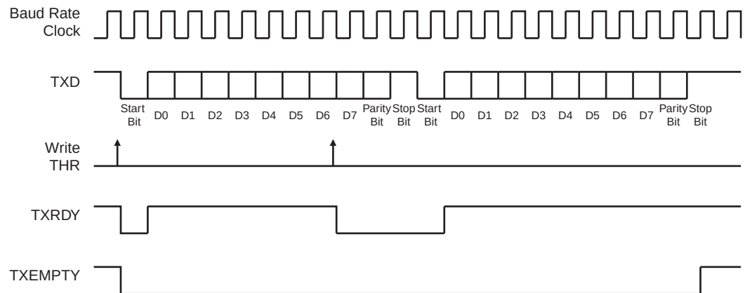
Figure 25-3. Transmitter Status
