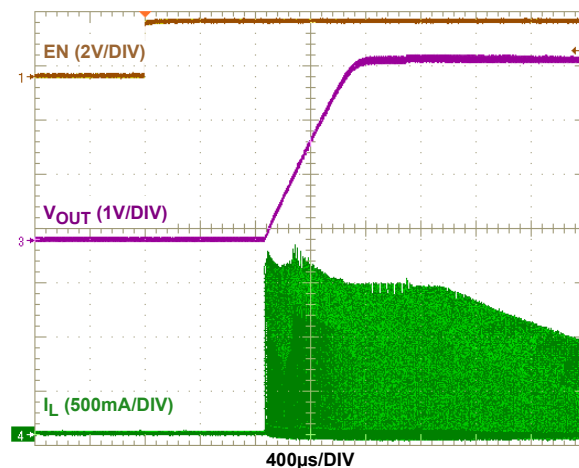
FIGURE 8. SOFT-START ( V_{IN} = 4V , V_{OUT} = 3.3V , 0.5A R_{LOAD} )
