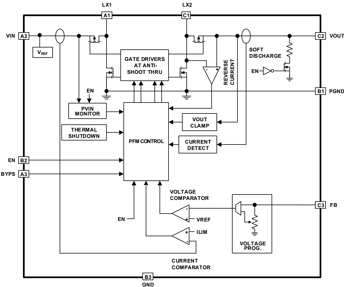
FIGURE 3. BLOCK DIAGRAM
