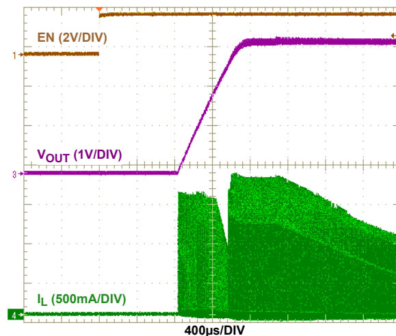
FIGURE 10. SOFT-START ( V_{IN} = 3V , V_{OUT} = 3.3V , 0.5A R_{LOAD} )
