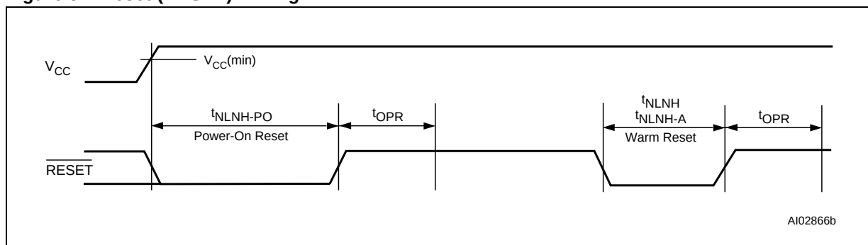
Figure 51. Reset (RESET) Timing
