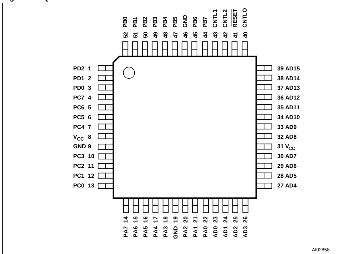
Figure 2. PQFP52 Connections
