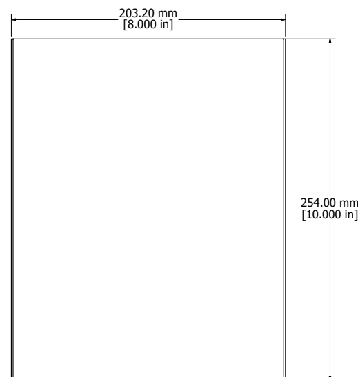
BOTTOM / TOP OF ENCLOSURE
