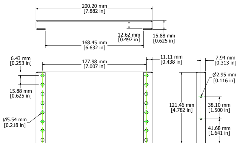
END PLATES
