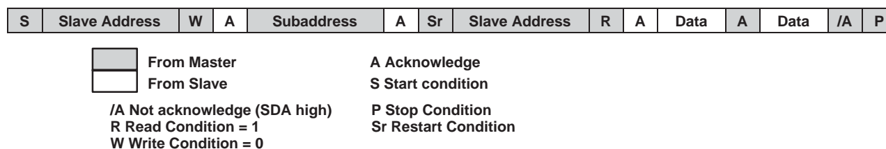
Figure 13. I 2 C Read Cycle
