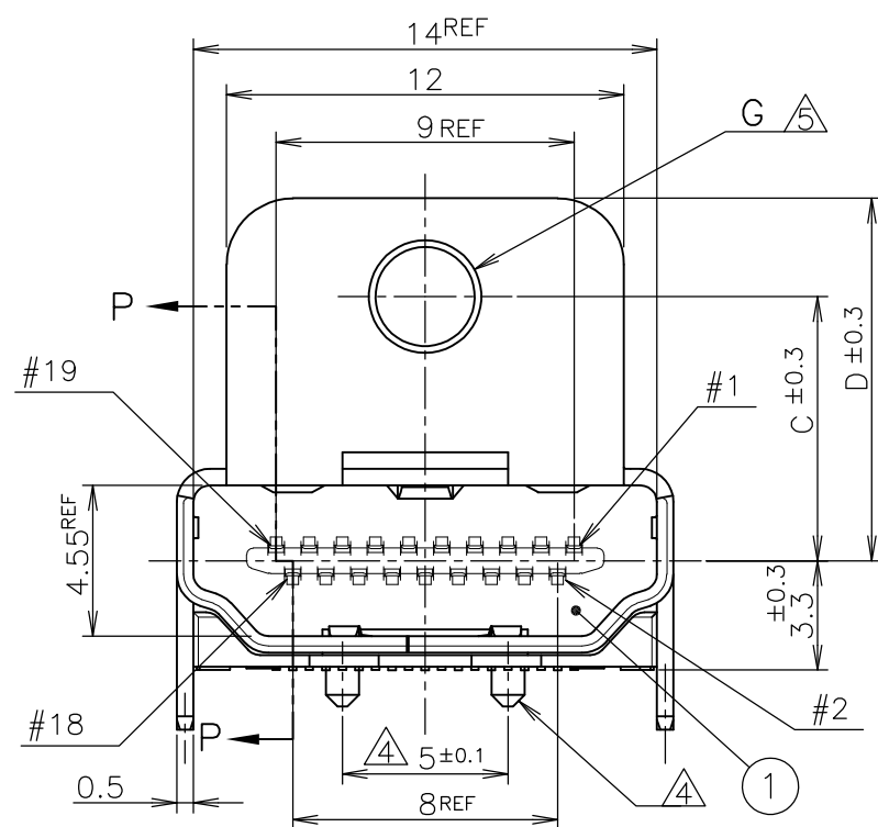
CONNECTOR WITH FLANGE TYPE
