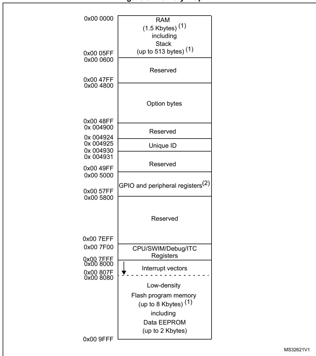
Figure 3. Memory map
