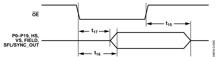
Figure 4. OE Timing
