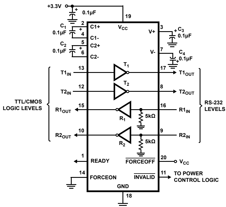
Figure 1. ICL3224E
