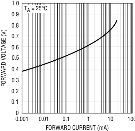
Forward Characteristics
