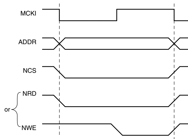
Figure 14. Early Read Protocol
