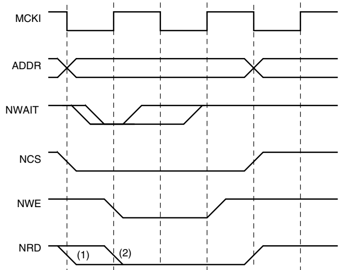
Figure 19. External Wait
