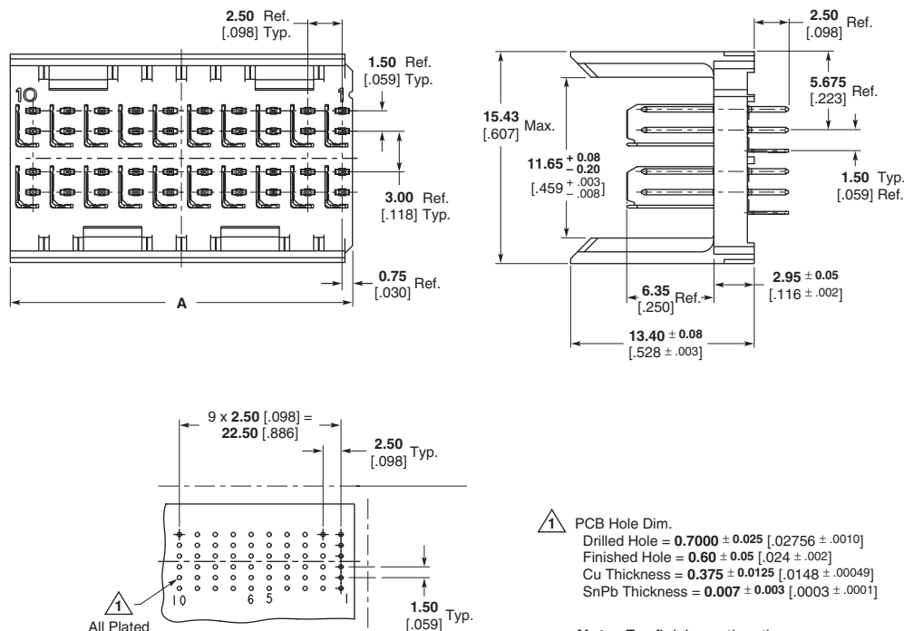
Recommended PC Board Layout Backplane
