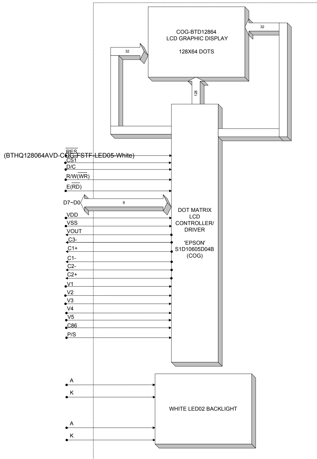
Figure 3: Block Diagram.
