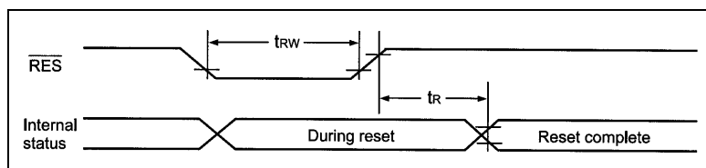
Figure 8: Reset Timing
