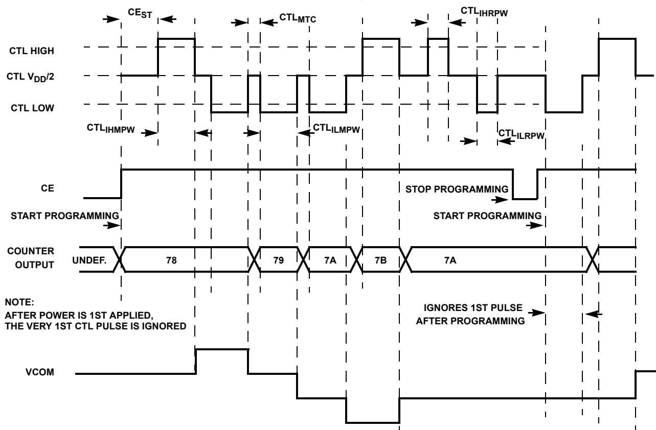
FIGURE 8. ISL45042 TIMING DIAGRAM
