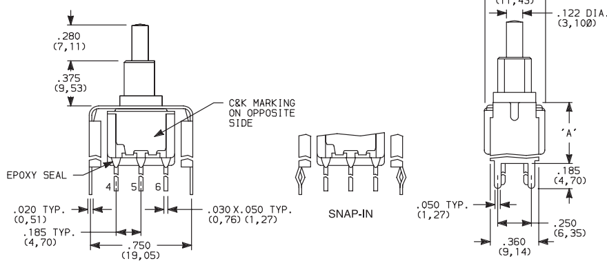
8261SH9_BE2 DPDT
