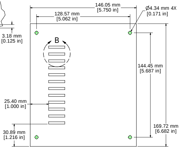
ENCLOSURE CASE - BOTTOM VIEW
