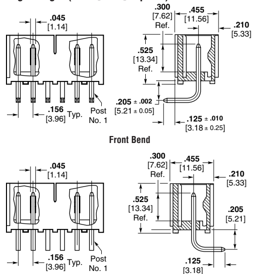
Rear Bend Edge of Board Recommended Mounting Hole Pattern for .062 [1.57] Thick PC Board Using a Right-Angle Header
