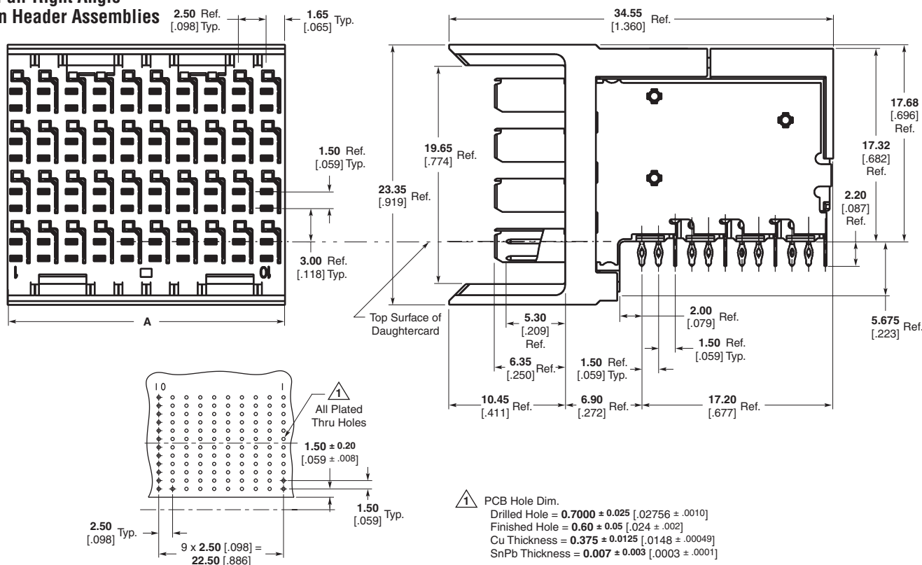
Recommended PCB Layout Component Side Shown
