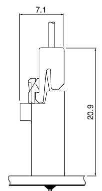
PAF Receptacle + PA high box type header
