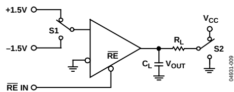
Figure 9. Receiver Enable/Disable
