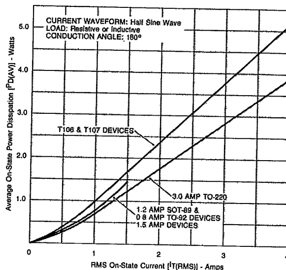
FIGURE 12 — Power Dissipation (Typical) vs RMS On-State Current
