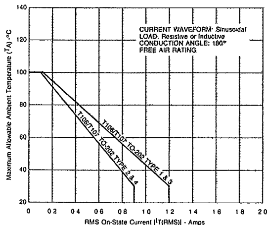
FIGURE 3C — Maximum Allowable Ambient Temperature vs RMS On-State Current
