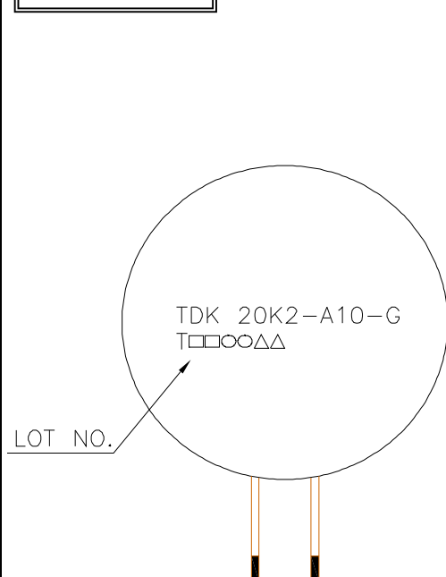
BOTTOM VIEW
