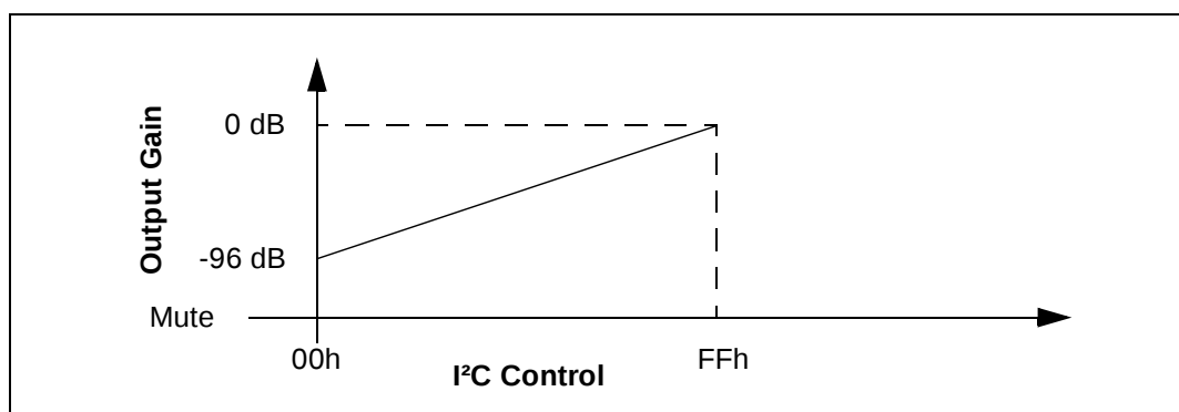
Figure 10: Volume Control
