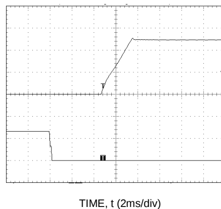
Figure 22. Typical Start-Up Characteristics from Remote ON/OFF.
