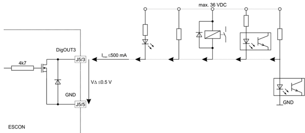
Figure 3-14 DigOUT3 Wiring Examples (analogously valid also for DigOUT4)
