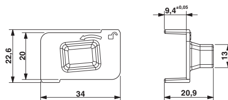
Sealing plug with locking for push-pull panel mounting frame
