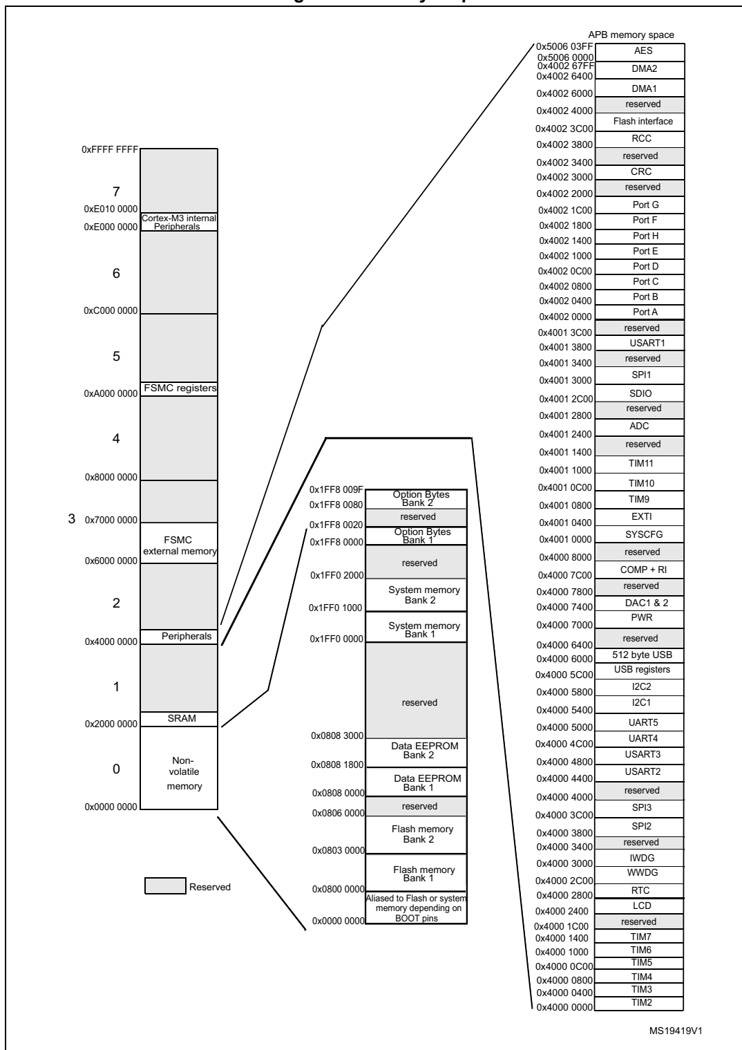
Figure 8. Memory map
