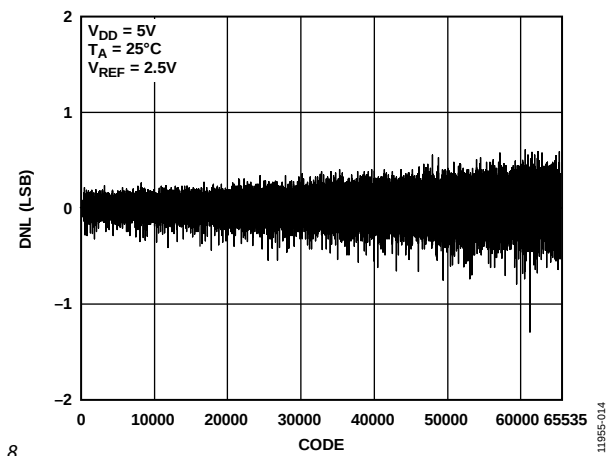
Figure 14. AD5683R/AD5683 DNL
