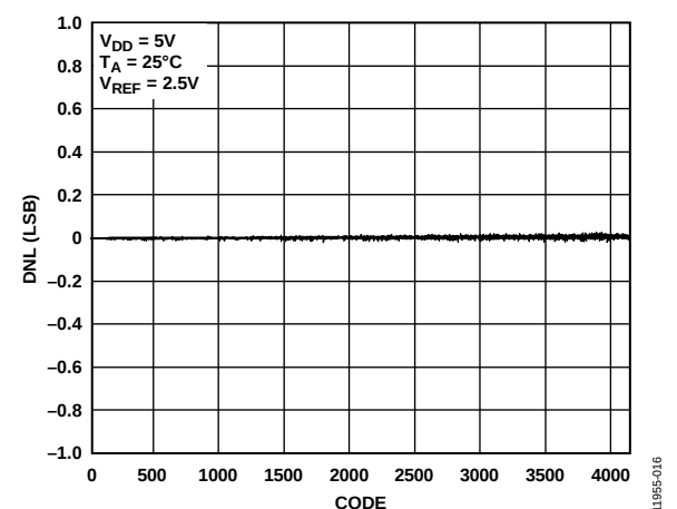
Figure 16. AD5681R DNL
