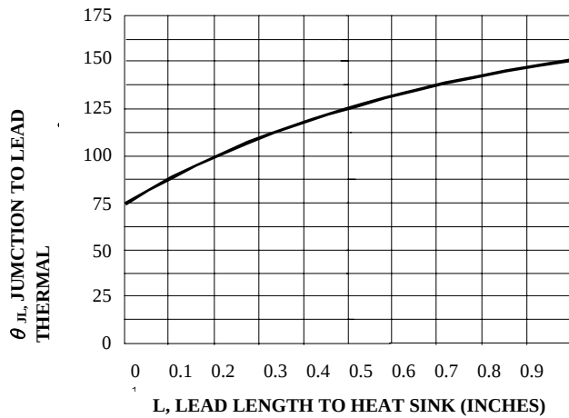
Figure 3. Typical Thermal Resistance versus Lead
