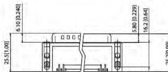
13.84mm[0.545"] Footprint
