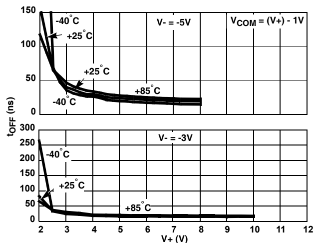
FIGURE 16. TURN - OFF TIME vs POSITIVE SUPPLY VOLTAGE
