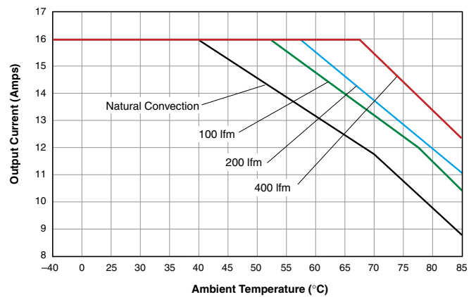
LSN-T/16-W3 Maximum Output Current vs. Ambient Temperature (V OUT = 3.3V, V IN = 5V)
