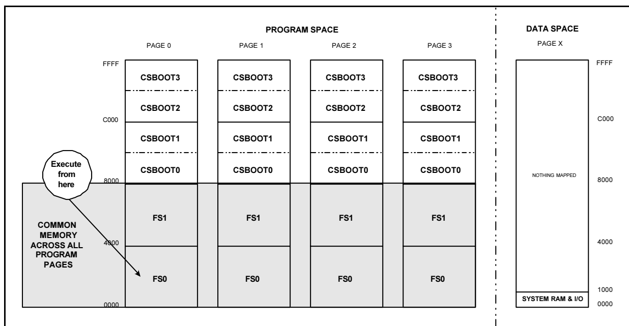
Figure 22 Memory locations after step 3 of memory swap
