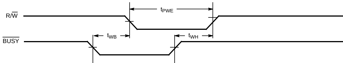
Figure 12. Write Timing with Busy Input (M/ \overline{\text{S}} =LOW)
