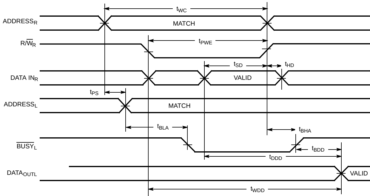
Figure 12. Write Timing with Busy Input (M/ \overline{\text{S}} =LOW)
