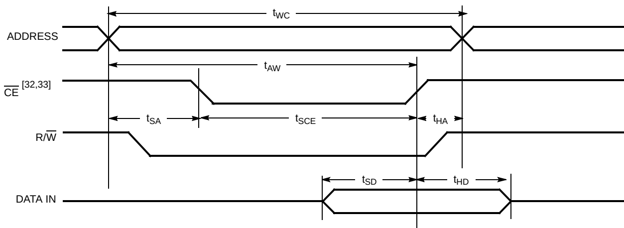
Figure 8. Write Cycle No. 2: \overline{CE} Controlled Timing [28, 29, 30, 34, 35]
