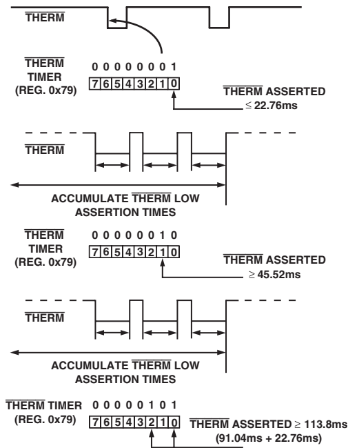
Figure 26. Understanding the THERM Timer
