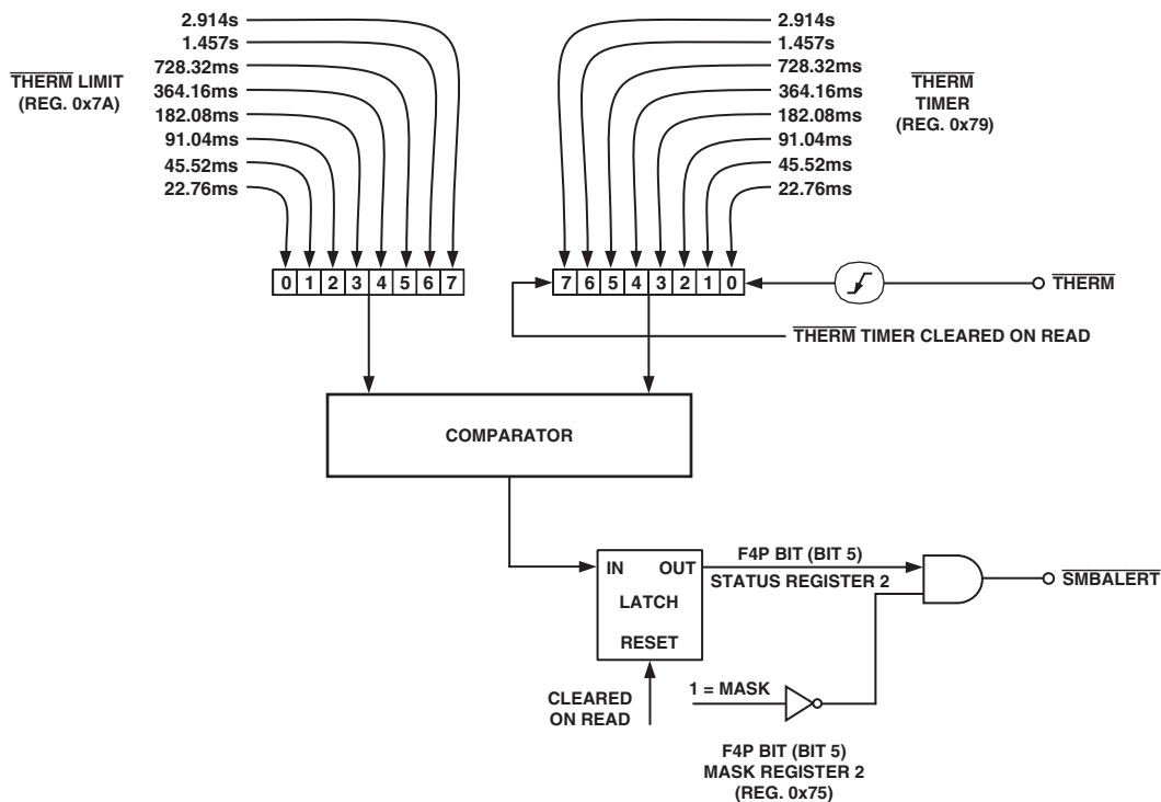
Figure 27. Functional Diagram of ADT7460's THERM Monitoring Circuitry
