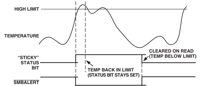
Figure 23. \overline{\text{SMBALERT}} and Status Bit Behavior
