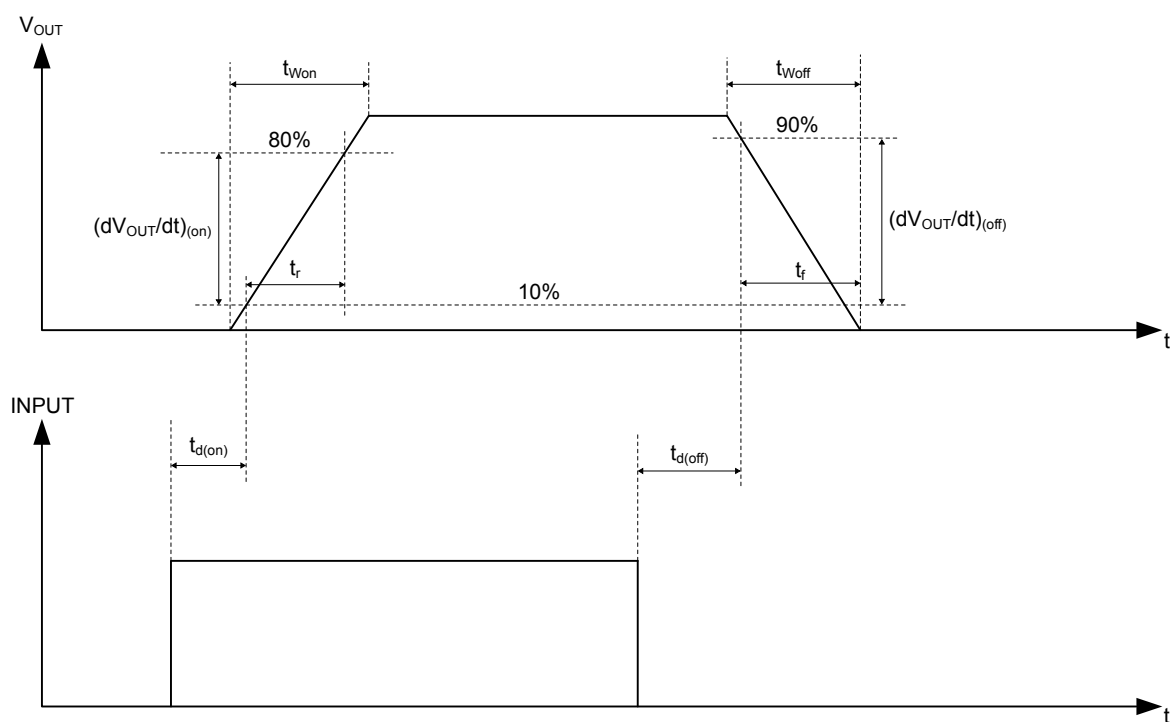
Figure 8. Switching characteristics
