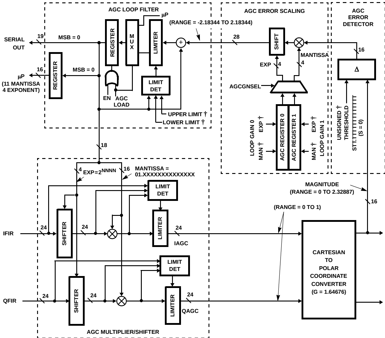
FIGURE 1. AGC FUNCTIONAL BLOCK DIAGRAM
