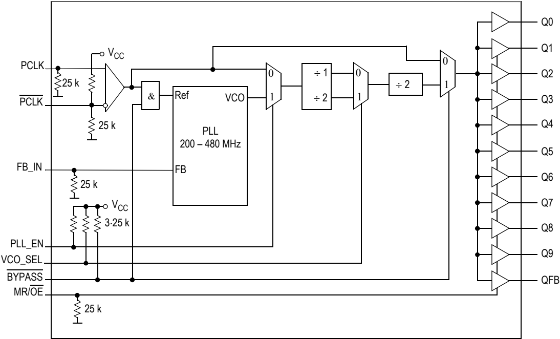
Figure 1. MPC9658 Logic Diagram
