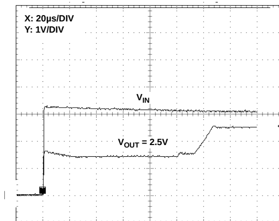
FIGURE 38. TURN-ON TIME
