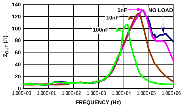
FIGURE 12. Z_{OUT} vs FREQUENCY
