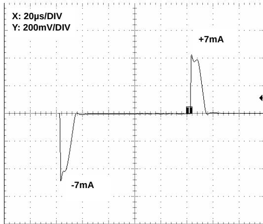
FIGURE 27. LOAD TRANSIENT RESPONSE, 0.001μF LOAD CAPACITANCE
