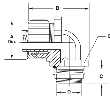
Sizes: 3/8", 1/2", 3/4", 1"
