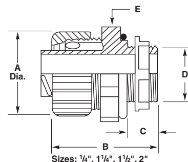
Sizes: 1/4", 1 1/4", 1 1/2", 2"
