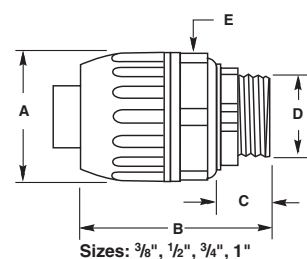
Sizes: 3/8", 1/2", 3/4", 1"
