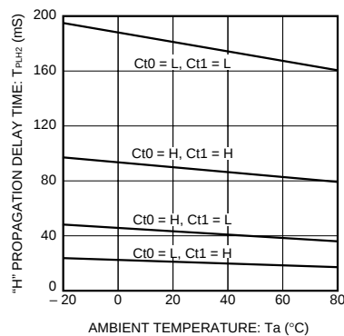
Fig. 6 Reset circuit 2 high level transmission delay time vs. ambient temperature
