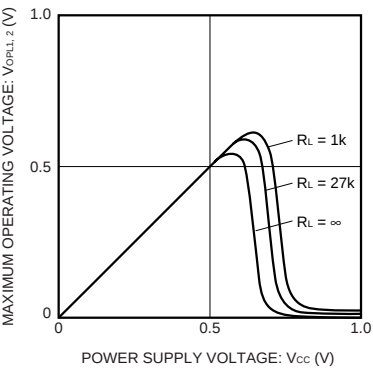
Fig. 7 Operation limit voltage vs. power supply voltage
