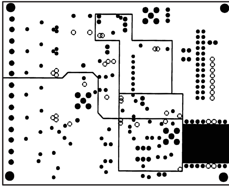
Internal Plane 2
