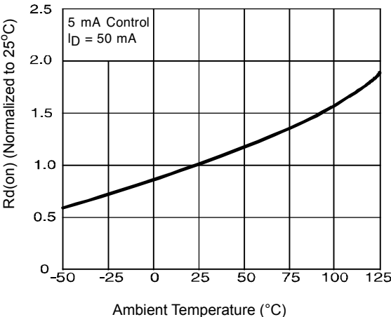
Figure 2. Typical On-Resistance
