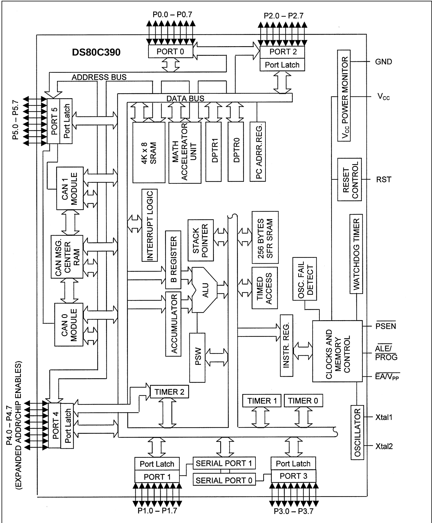
Figure 28. Block Diagram
