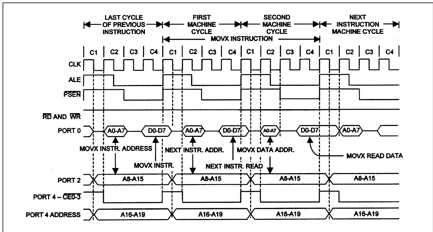
Figure 5. Multiplexed 2-Cycle Data Memory \overline{CE0-3} Read
