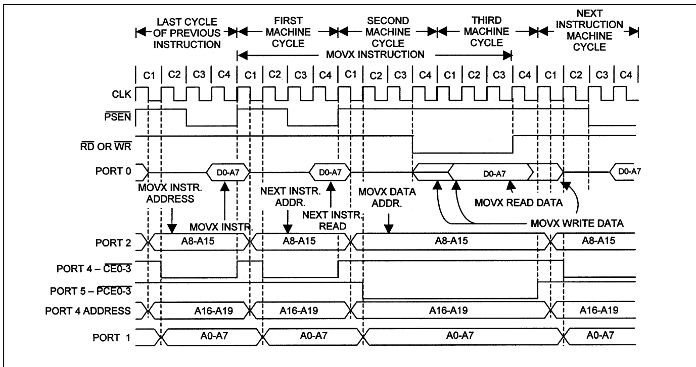
Figure 19. Nonmultiplexed 3-Cycle Data Memory \overline{PEC0-3} Read or Write
