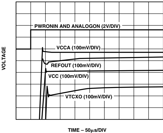
TPC 10. Turn-On Transients, Maximum Loads
