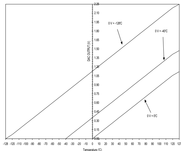
Figure 14. DAC Output vs Temperature, V_{REF} = 2.25\text{ V}
