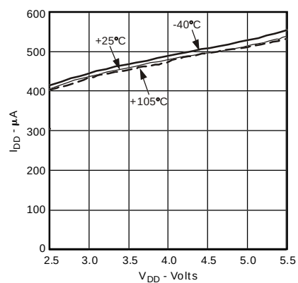
TPC 13. Supply Current vs. Supply Voltage
