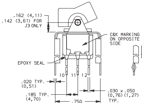
SNAP-IN
